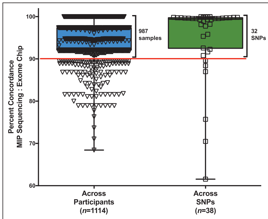
Figure 2. Concordance of variants identified from molecular inversion probe (MIP) sequencing with exome chip genotyping. Single-nucleotide variants identified in the targeted regions by MIP sequencing were compared with the discovery of those variants by genotyping on the exome chip in a subset of 1114 participants who were included in both variant discovery efforts. A total of 38 single-nucleotide polymorphisms (SNPs) that were included in the exome chip were found to overlap the targeted regions by MIPs. Box plot on the (left) shows the percentage of total SNPs that were found by both discovery methods for each individual ( n=1114 participants). Box plot on the (right) shows the percentage of individuals for which a given SNP was found to be concordant across the 2 discovery methods ( n=38 SNPs). Red line indicates those samples (left) and SNPs (right) for which concordance between MIP sequencing and the exome chip genotyping was >90\% . Thirty-two of 38 SNPs (84.2%) overlapping on the exome array were called with >90\% concordance across all participants. Nine hundred eighty-seven of 1114 participants (88.6%) demonstrated >90\% concordance of all genotyped SNPs.
