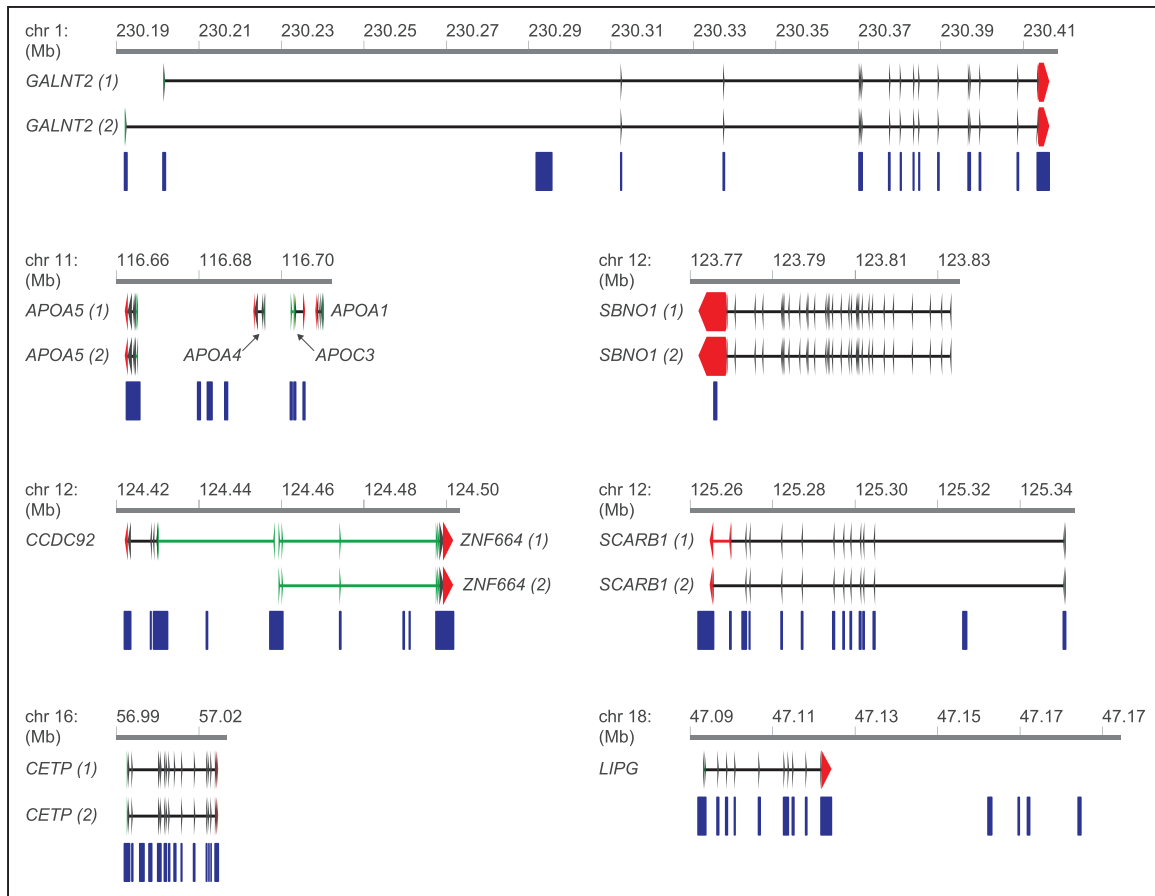
Figure 1. Candidate gene regions for molecular inversion probe (MIP) targeted sequencing. All coordinates correspond to genomic build GRC37/hg19. Blue boxes correspond to MIP target locations.
